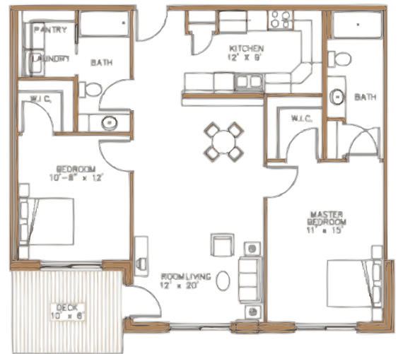
Two Bedroom 1,003 sq.ft.
